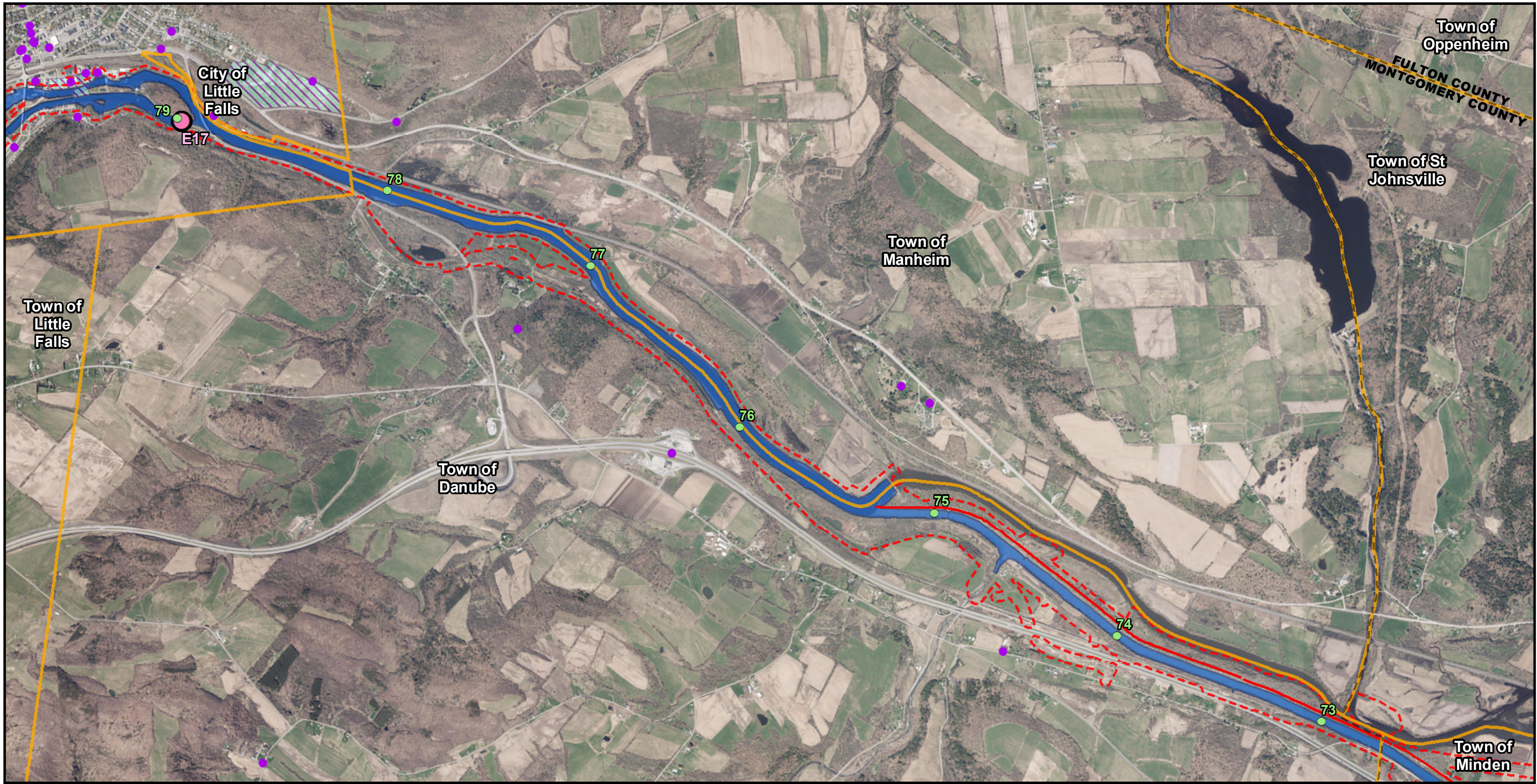
EARTHEN EMBANKMENT INTEGRITY PROGRAM Figure 38H: Potential Contamination Sources Town of Manheim Date: 11/6/2018
